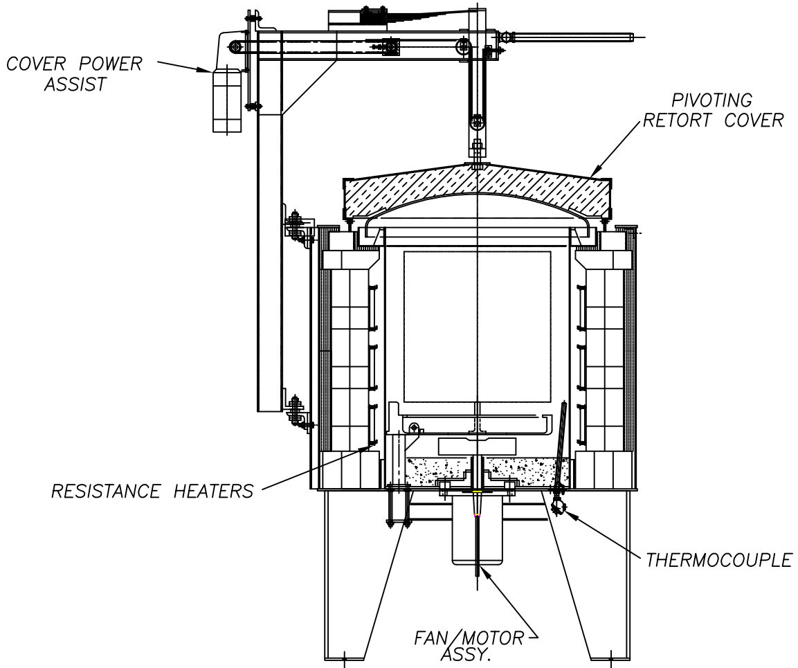
UPTON PIT TYPE FURNACE U-PE
