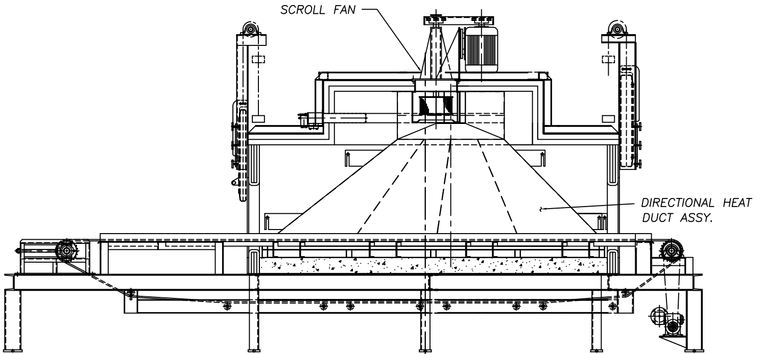
UPTON DUAL BELT TYPE CONTINUOUS FURNACE U-CONT
