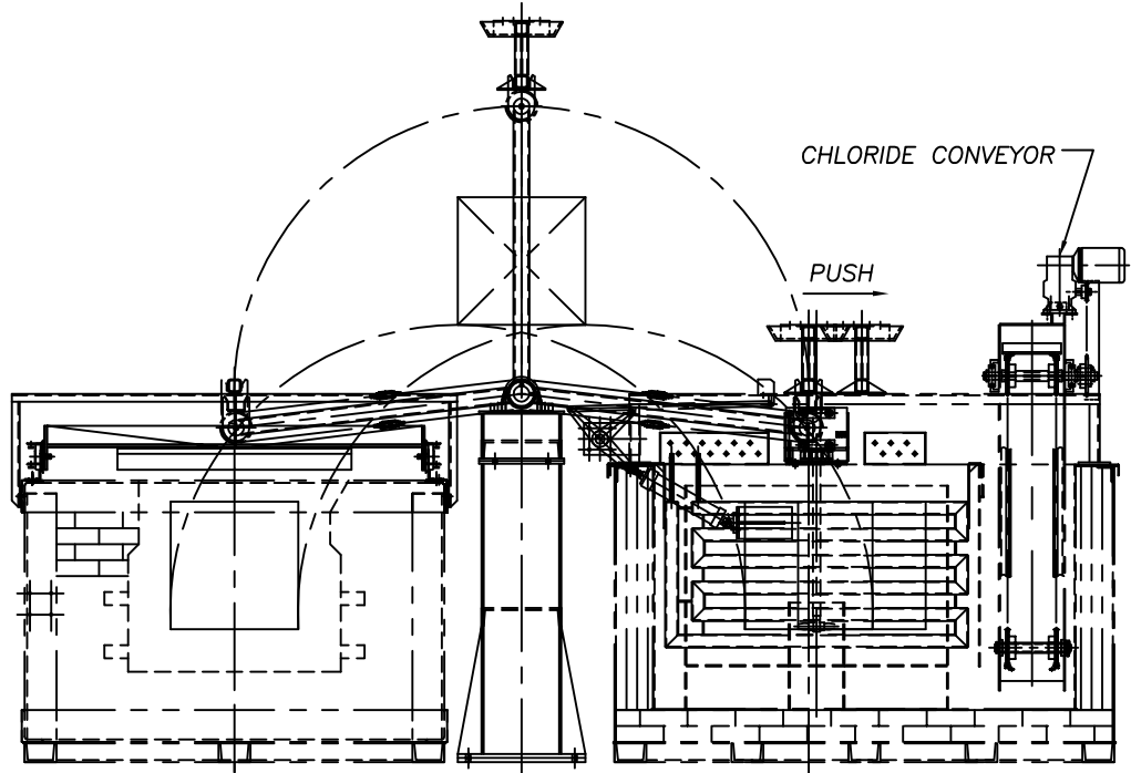
CERAMIC SALT BATH FURNACE
