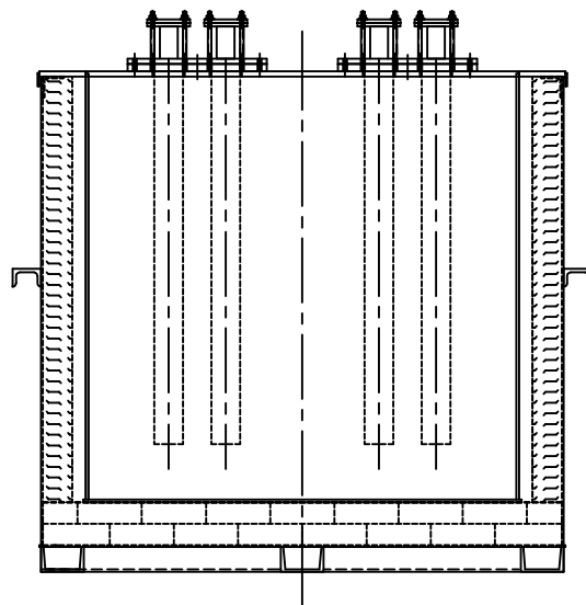
INTERNALLY HEATED SALT BATH FURNACE U-DS
