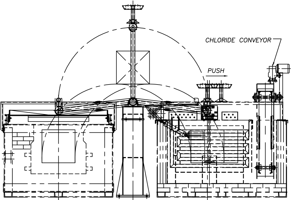
CERAMIC SALT BATH FURNACE
